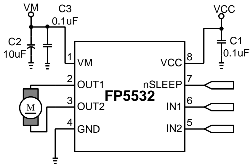
Figure 2. DC Motor Application Circuit for SOP Packages
