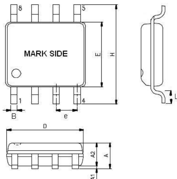
SOP- 8 Package (Unit: mm)
